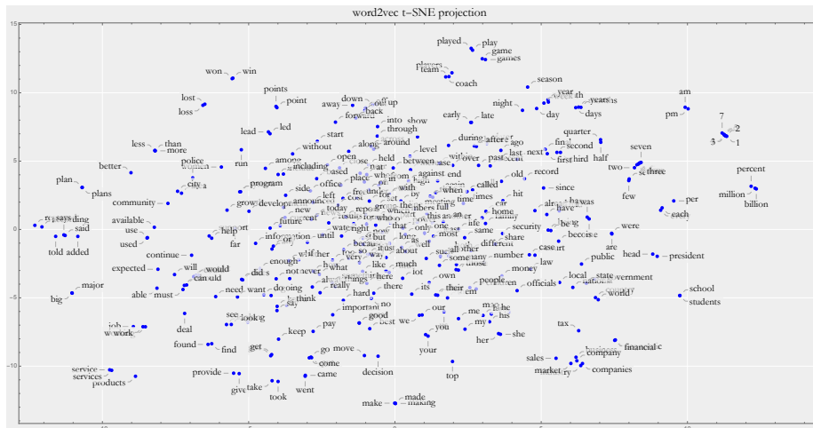
Figure 1: T-SNE two-dimensional projection of the word2vec vectors representing a selection of the most frequent words in its training corpus.
