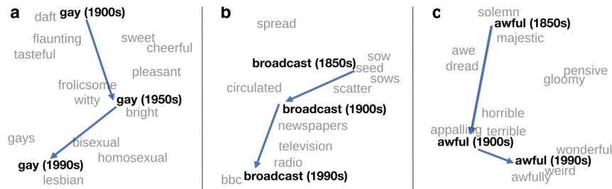
Figure 6: Visualization of semantic change based on word2vec. Credit: Hamilton et al. (2016).
