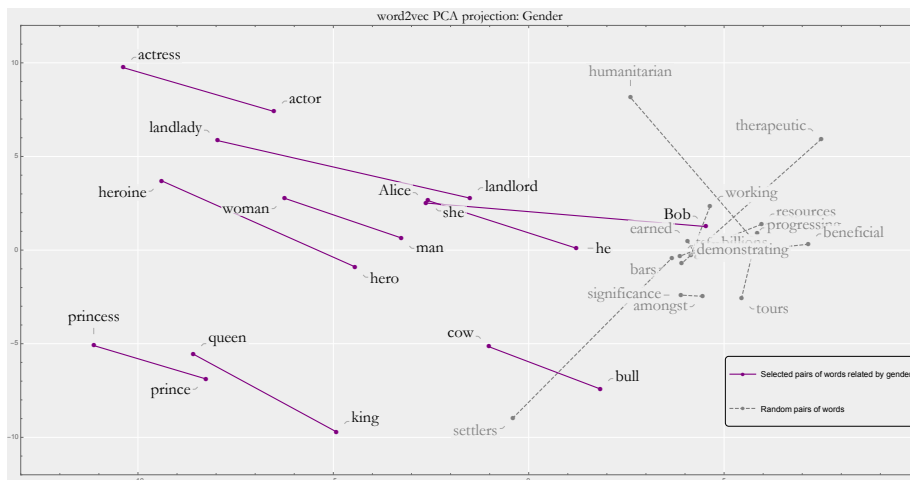
Figure 2: Offset representing the gender relation, revealed in the embedding space by a PCA projection.
