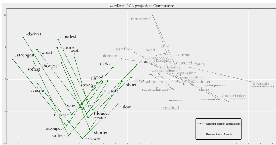
Figure 3: Pattern in the embedding space (word2vec) corresponding to the comparative category (base, comparative and superlative forms).
