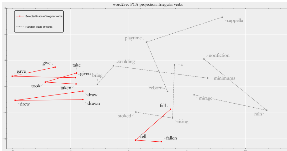
Figure 4: Pattern in the embedding space (word2vec) corresponding to conjugation of irregular verbs.
